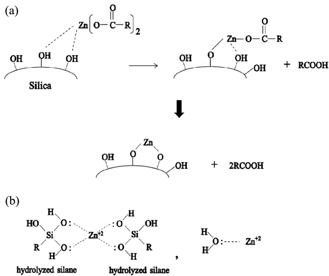
Figure 5. (a) Zinc ion reaction with hydroxyl group on silica surface /redraw from ref.19; (b) Zinc ion interaction with hydroxyl group in silane.
