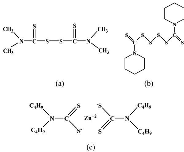
Figure 1. Chemical structure of thiram type accelerators: (a) TMTD; (b) DPTT; (c) ZDBC.
