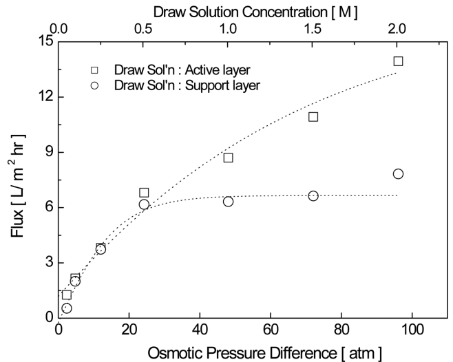
Fig. 3. Variation of water flux with osmotic pressure difference for a variety of draw solution concentrations.
