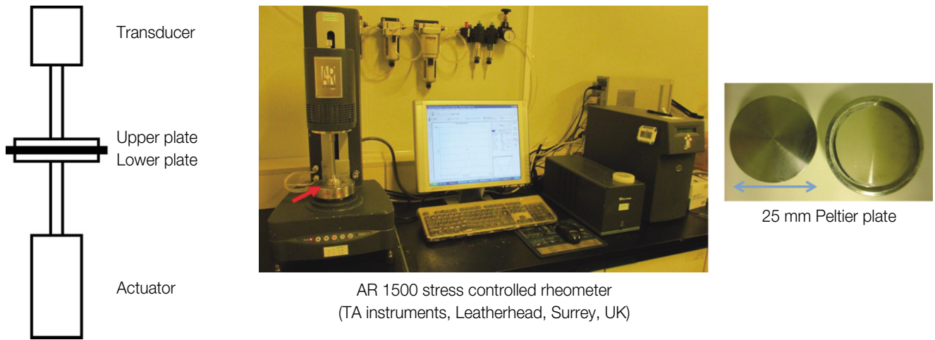
Fig. 1. Dynamic oscillatory time sweep testing involves the application strain to a resin cement material and to record the resultant stress. The phase angle ( \delta ) and the ratio of stress amplitude and strain amplitude allow the calculation of the shear storage modulus ( G' ), loss modulus ( G'' ), loss tangent ( \tan \delta ) and other rheological variables.
