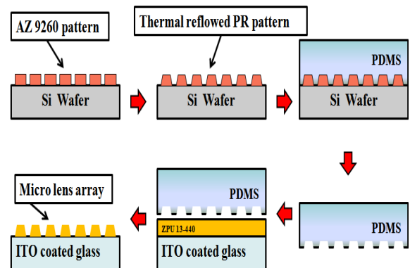
Fig. 2. Fabrication process of microlens array.
