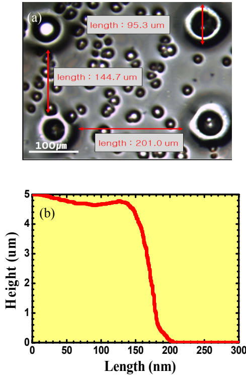
Fig. 3. (a) Picture of microlens array after thermal reflow taken by optical microscope (Olympus Co., Ltd.) and (b) height of microlens measured by alpha step 200 (Tencor Co., Ltd.).
