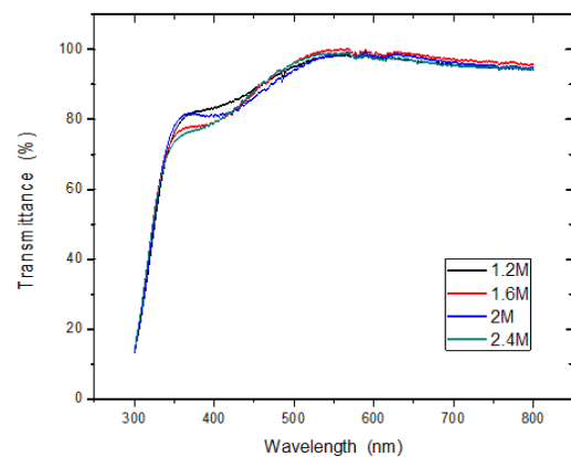
Fig. 5. The transmittance of ZnS film with ammonia solutions molarity.
