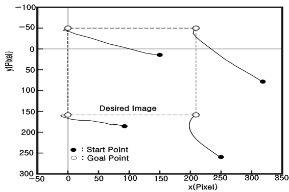
Fig. 5 Image coordinates of a particular point(Monocular)
