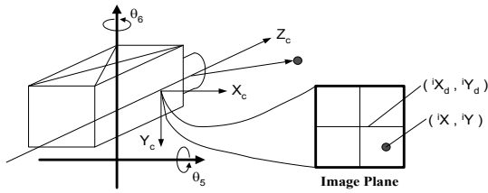
Fig. 4 Camera arrays of the robot wrist joint
