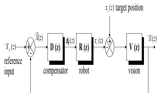
Fig. 3 Vision system of the visual feedback control system block diagram.
