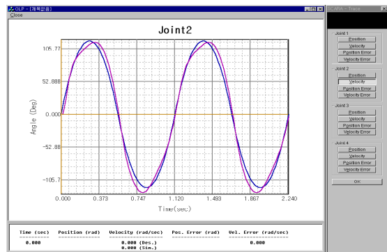
Fig. 2 Simulation trajectory tracking.
