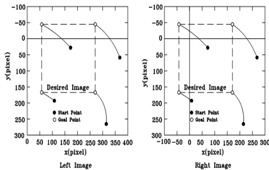
Fig. 6 Image coordinates of a particular point(Stereo)
