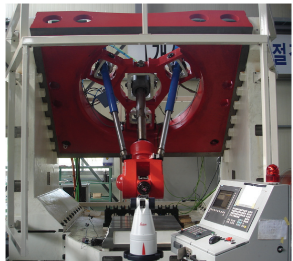
Fig. 4. Prototype of a 5-axis hybrid machine tool.
