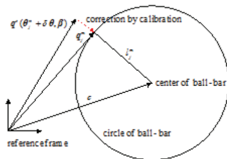
Fig. 3. Outline of the calibration methods using a ball-bar.
