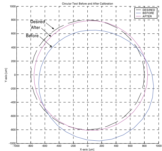
Fig. 5. Circular test before and after calibration.
