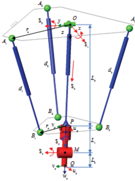
Fig. 2. Kinematic parameters of the machine tool.
