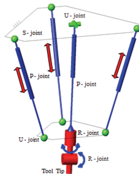
Fig. 1. Structure of the hybrid-kinematic machine tool.
