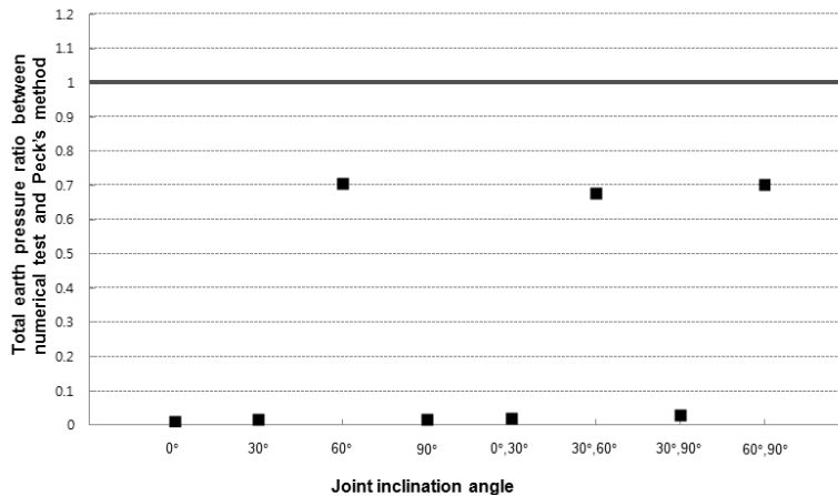
Fig. 7. Total Earth Pressure Ratio Between Induced Earth Pressure and Peck's Earth Pressure (Hard Rock)
