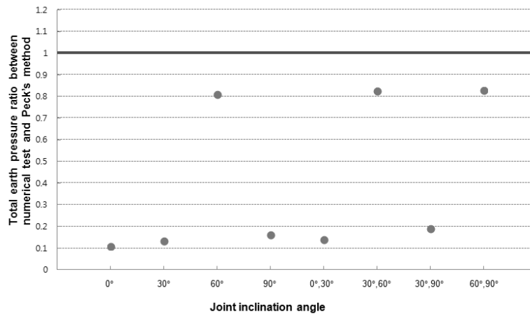
Fig. 9. Total Earth Pressure Ratio Between Induced Earth Pressure and Peck's Earth Pressure (Slightly Weathered Rock)
