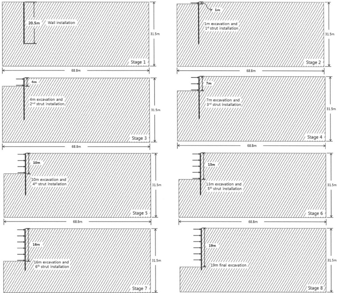
Fig. 4. Sequential Excavation Stages in the Numerical Simulation (A Case of Joint Inclination 60°)
