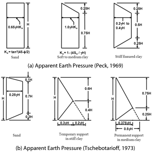
Fig. 1. Apparent Earth Pressure in Soil Ground
