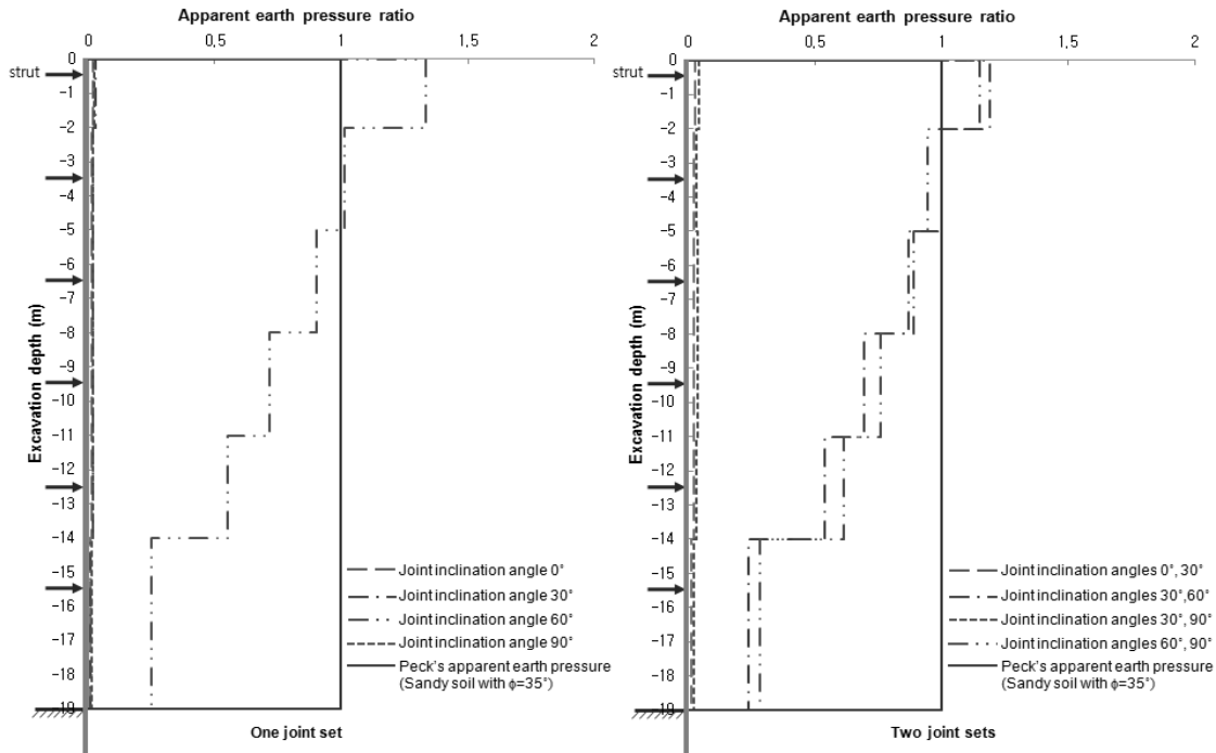
Fig. 6. Earth Pressure Distribution and Magnitude in Hard Rock
