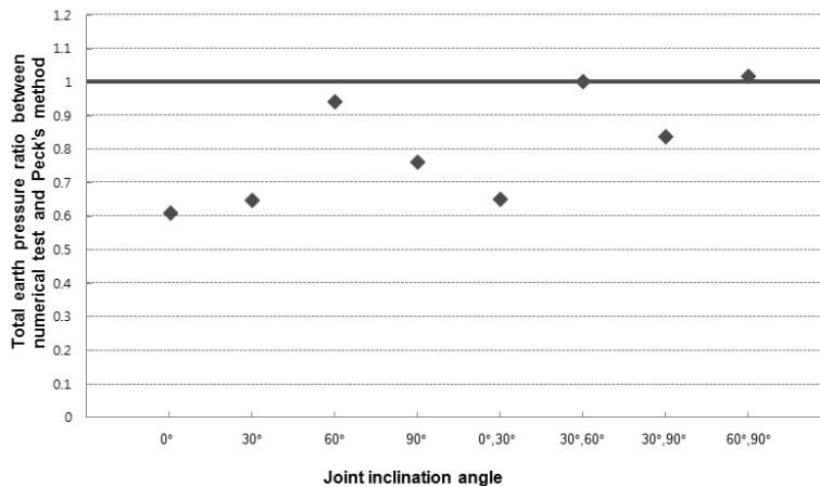
Fig. 11. Total Earth Pressure Ratio Between Induced Earth Pressure and Peck's Earth Pressure (Moderately Weathered Rock)
