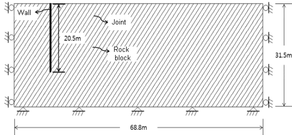
Fig. 2. Numerical Modeling (A Case of One Joint Set, Joint Spacing of 1 m, and Joint Inclination of 60°)
