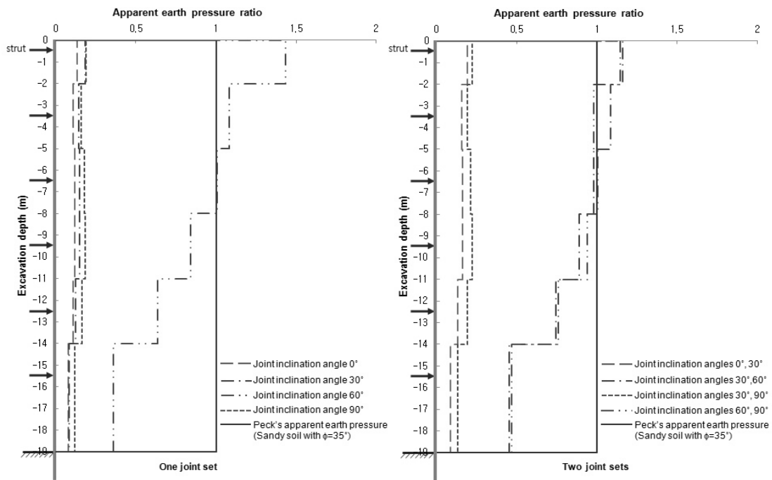
Fig. 8. Earth Pressure Distribution and Magnitude in Slightly Weathered Rock
