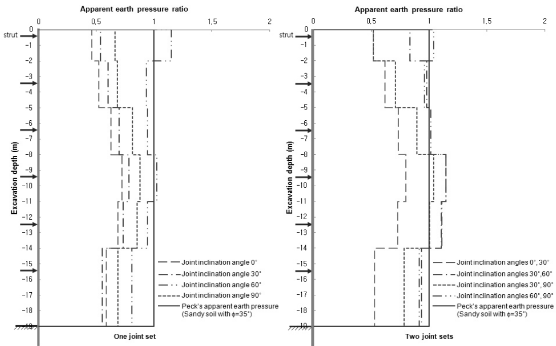
Fig. 10. Earth Pressure Distribution and Magnitude in Moderately Weathered Rock
