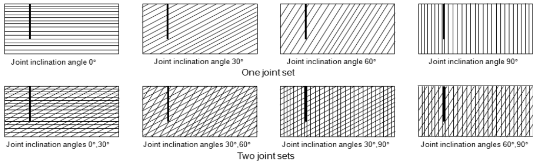
Fig. 3. Modeling of Joint Sets
