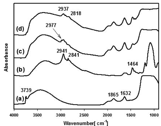
Figure 2. FTIR spectra of (a) pristine silica; (b) pure BTPED; (c) modified silica with ( \# of Si(OCH 3 ) 3 mol)/( \# of SiOH mol) = 1; (d) ( \# of Si(OCH 3 ) 3 mol)/( \# of SiOH mol) = 2.
