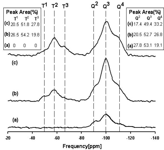
Figure 5. 29 Si NMR spectra of (a) pristine silica; (b) modified silica with (# of Si(OCH 3 ) 3 mol)/(# of SiOH mol) = 0.5; (c) (# of Si(OCH 3 ) 3 mol)/(# of SiOH mol) = 1.
