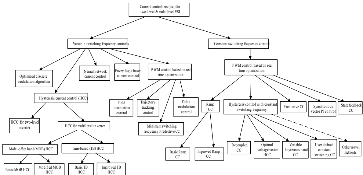
Fig. 3. Classification of current control techniques based on variable & constant switching frequency regulation.
