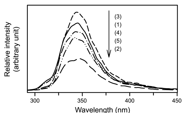
Figure 3. Steady-state fluorescence emission spectra of quercetin in various 3% AOT reverse micelles; (1) R = 0 (—), (2) R = 4.0 (---), (3) R = 10.0 (·····), (4) R = 20.0 (-·-·-), (5) R = 30.0 (- - - - -).
