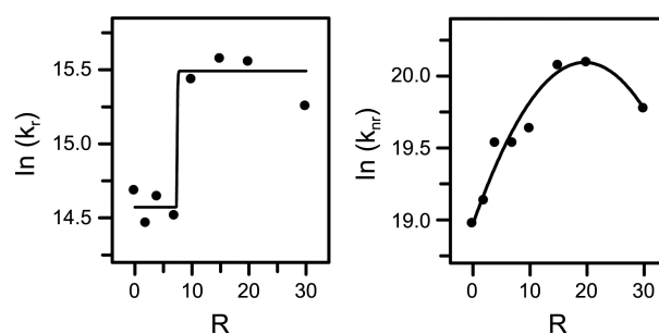
Figure 4. Logarithms of the radiative rate constants, k_r and nonradiative rate constants, k_{nr} , plotted as a function of the molar ratio of water to AOT, R , in the 3% AOT reverse micelle. The solid lines are the best polynomial regression fit to the data.
