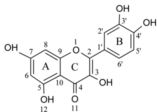
Scheme 1. The molecular structure of quercetin.
