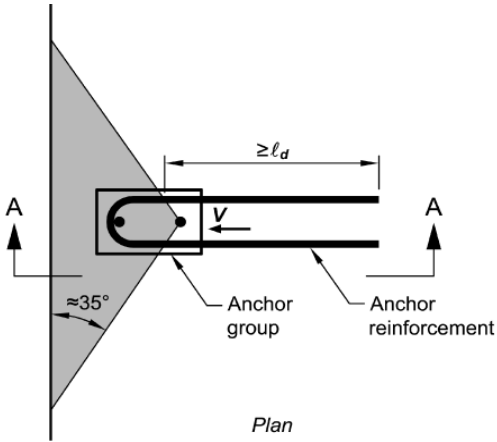
Fig. 1. Hairpin reinforcement [3]
