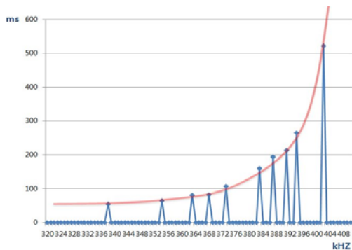
Figure 8: Charging time of capacitor Vs. frequency ( C_b = 34\mu\text{F} , V_{max} = 240\text{V} , L_{m2} = 4.5\text{mH} )
