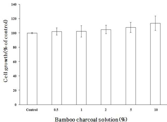
Fig. 1. Effect of bamboo charcoal on the viability of HGF
