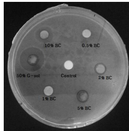
Fig. 3. Antibacterial activity of ratio bamboo charcoal against S. mutans
