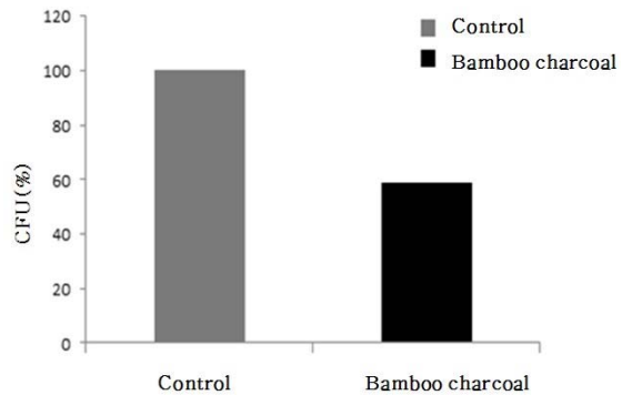
Fig. 2. Variable cell count of S. mutans in bamboo charcoal solution
