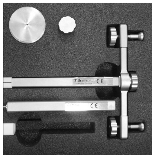
Fig. 4. Image of Winston Lutz Test Tool Sets.
