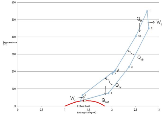
Fig. 4 T-S Diagram of Recompressing S-CO 2 Cycle Layout
