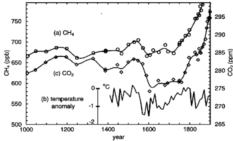
Figure 1. Methane and carbon dioxide variations during the pre-Anthropocene. Curve (a) Methane mixing ratios from Antarctic and Greenland ice-cores. Curve (b) Temperature anomaly for northern hemispheric summers, decadal means, referenced to 1860–1959. Curve (c) Ice core CO 2 record with 75-year smoothing spline fit. Source: D. M. Etheridge et al., “Atmospheric Methane between 1000 A.D. and Present,” 15985.
