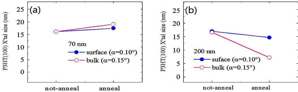
Figure 2. (a) and (b) are the P3HT(100) crystal size from GIWAXS data in 70nm and 200nm thick films, respectively. The information of the surface region was obtained when the x-ray incident angle \alpha was 0.10^\circ (blue lines), while the information from the bulk region was obtained in case of \alpha = 0.15^\circ (red lines).
