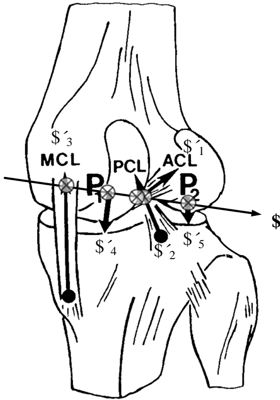
Figure 1. Five constraints \$' s are collectively reciprocal to the instantaneous screw axis \$ . The instantaneous motion of the knee is guided by the constraints of the anterior cruciate ligaments (ACL), posterior cruciate ligament (PCL), medial collateral ligament (MCL), and articular contact in the medial ( P_1 ) and lateral ( P_2 ) compartments. Note that no combination of the constraint forces that might be generated at the \$ will result in a rotation at the \$ , and no angular velocity about the \$ will cause the constraint force to do any work at the points on the medial and lateral contacts. (Adapted from the original figure published in Kim and Kohles [24].)
