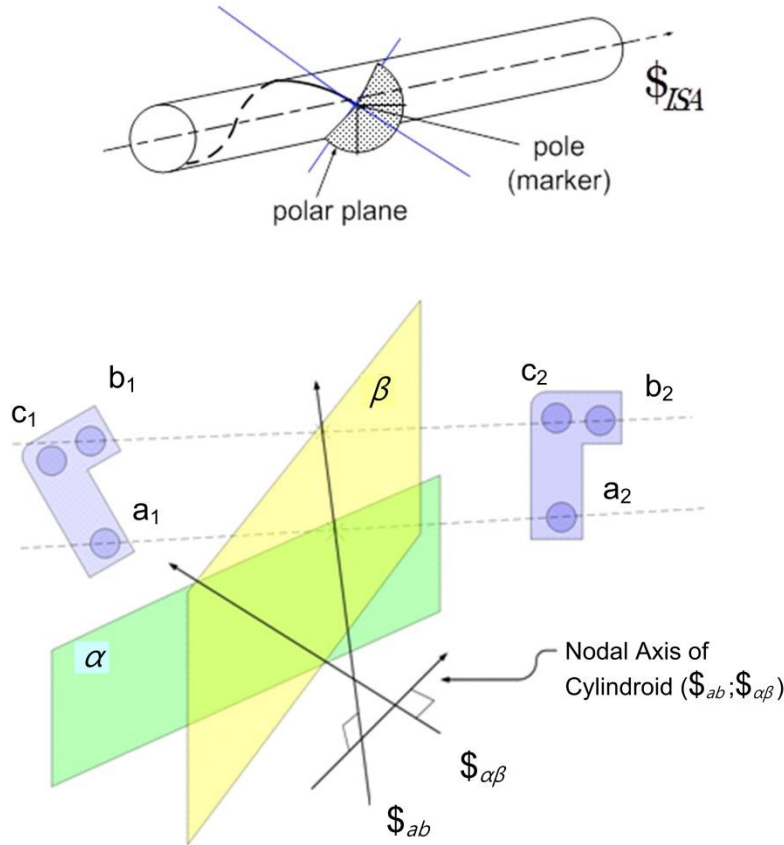
Figure 3. A special line complex is that defined by a single twist \$ISA . Every marker point of the segment has its velocity vector tangential to the helix that passes through it. The pattern of this velocity vector is a helicoidal velocity field. Each marker point that does not coincide with the twist axis of \$ISA is referred to as a pole. Associated with each pole is its corresponding polar plane. Shown are a polar plane and its corresponding pole as defined by the instantaneous screw axis \$ISA . The ISA \$ISA used to transform the marker set (a_1, b_1, c_1) to (a_2, b_2, c_2) must be determined from cylindroids (\$ab; \$\alpha\beta) . \$_{\alpha\beta} and \$_{\alpha\beta} are two twists of zero pitch on the cylindroid (\$ab; \$\alpha\beta) .
