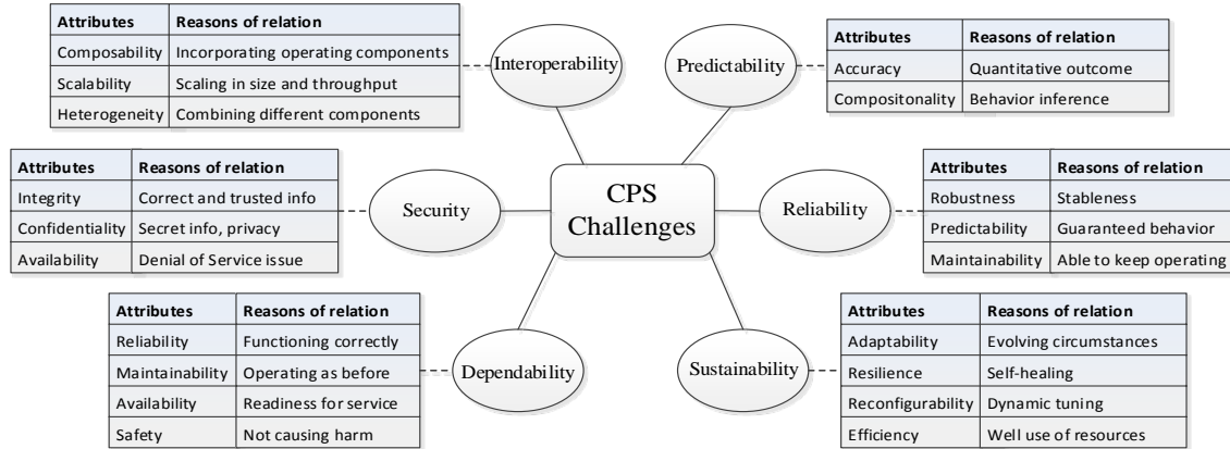
Fig. 3. CPS Challenges
