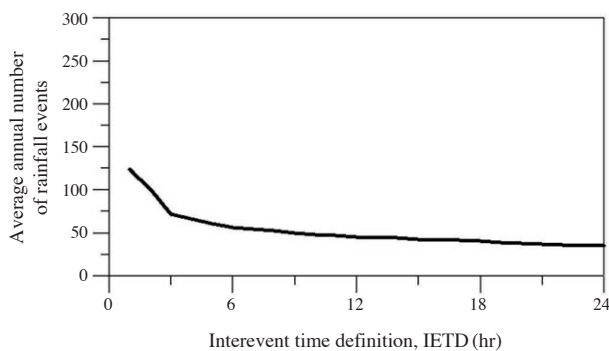
Fig. 4. Average annual number of rainfall events, in Seoul, Korea.
