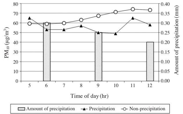
Fig. 6. Example of method for analysis of effect of precipitation scavenging on pollutant concentrations.
