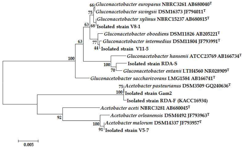
Fig. 1. Phylogenetic tree based on 16S rRNA sequences showing the positions of the acetic acid bacteria isolated from different kind of vinegar.
