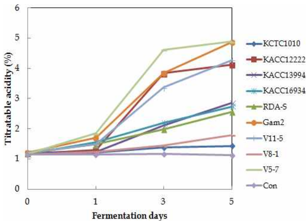
Fig. 2. Acetic acid production by isolated acetic acid bacteria and type strains.
