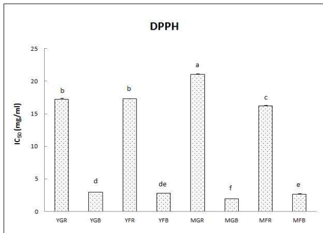
Fig. 2. Changes of DPPH radical scavenging activity in methanolic extract of Peucedanum japonicum Thunb.
