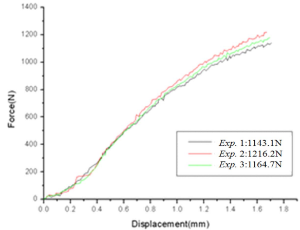
Fig. 8. Bending force-displacement curves
