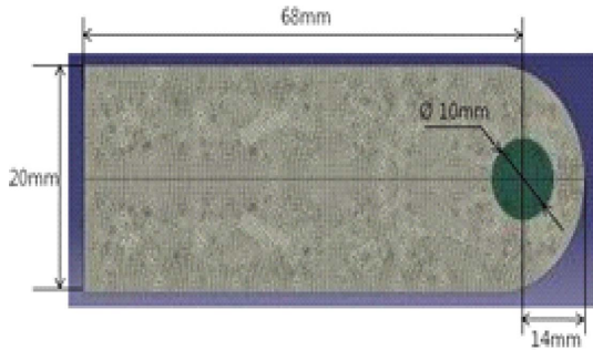
Fig. 9. Geometry and size of FEA model
