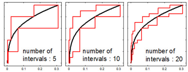
Fig. 5 Comparison between probability method and evidence theory with different numbers of intervals
