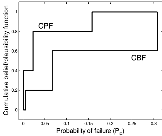
(b) cumulative plausibility and belief functions of the probability of failure
