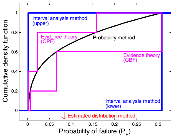
Fig. 6 CDF of the probability of failure
