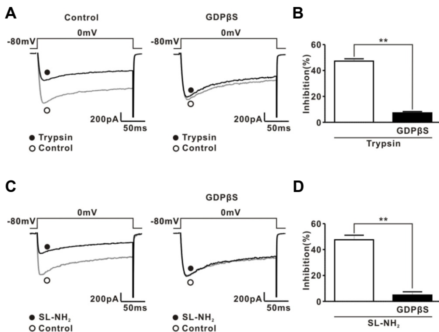
Fig. 2. Effect of GDPβS on PAR-2 agonist-induced I_{Ca} inhibition. (A) Left , a representative trace showing the effect of trypsin (30 nM) on I_{Ca} . Open (○) and filled circles (●) indicate I_{Ca} before and after trypsin application, respectively. Right , a representative trace showing the effect of trypsin (30 nM) on I_{Ca} with GDPβS (2 mM) in the pipette solution. Trypsin was applied to rat CG neurons after 7 min dialysis with GDPβS in the pipette solution. (B) Summary showing the effect of GDPβS on trypsin-induced I_{Ca} inhibition. (C) Left , a representative trace showing the effect of SL-NH 2 (100 μM) on I_{Ca} . Open (○) and filled circles (●) indicate I_{Ca} before and after SL-NH 2 application, respectively. Right , a representative trace showing the effect of SL-NH 2 (100 μM) on I_{Ca} with GDPβS (2 mM) in the pipette solution. SL-NH 2 was applied to rat CG neurons after 7 min dialysis with GDPβS in the pipette solution. (D) Summary showing the effect of GDPβS on SL-NH 2 -induced I_{Ca} inhibition.
