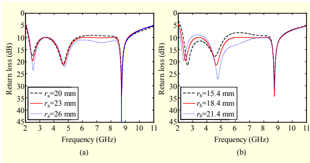
Fig. 2. Simulated return loss of unfolded, elliptical patch with different values of (a) r_a and (b) r_b .
