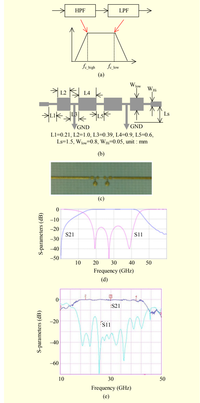
Fig. 7. Designed wideband IF BPF: (a) block diagram, (b) dimensions, (c) photograph, (d) simulated S-parameters, and (e) measured S-parameters.
