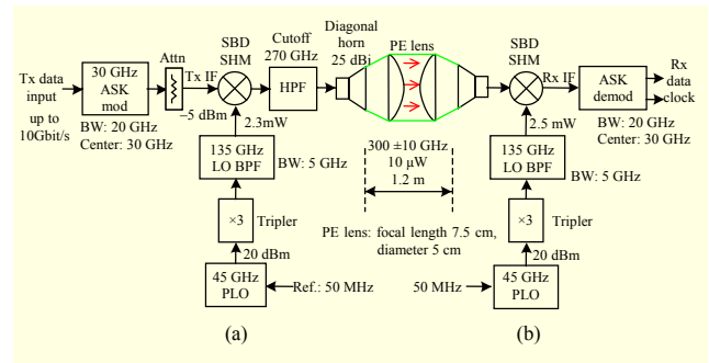
Fig. 1. Block diagram of proposed 10-Gbit/s wireless communication system at 300 GHz : (a) transmitter and (b) receiver.
