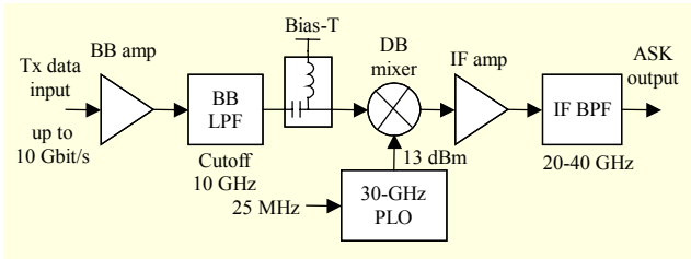
Fig. 5. Block diagram of 30-GHz ASK modulator.
