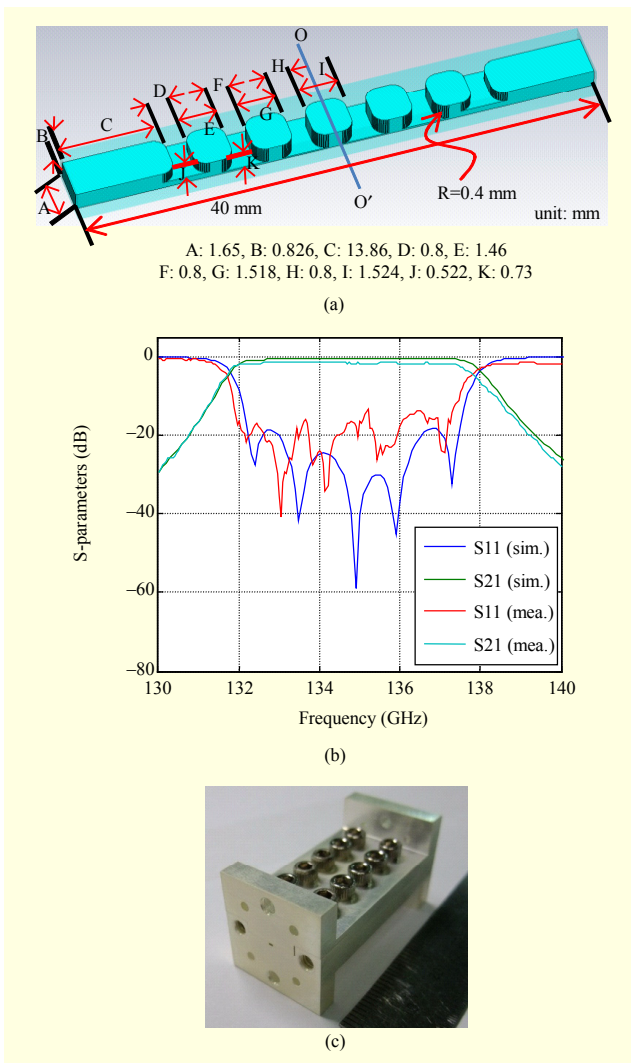
Fig. 9. Designed 135-GHz LO BPF: (a) dimensions, (b) simulated and measured S-parameters, and (c) photograph of device.
