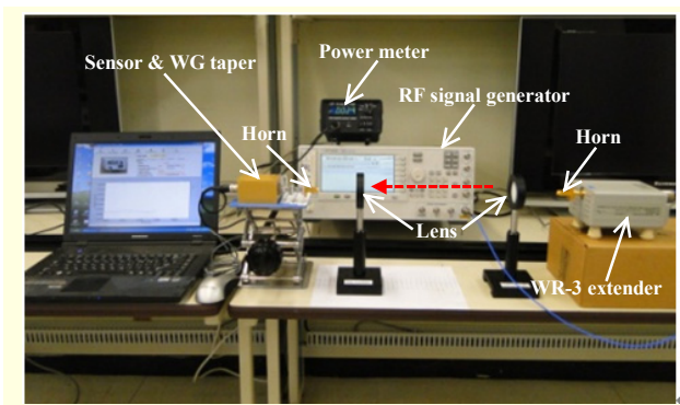
Fig. 17. Experimental setup used to measure effective antenna gain.
