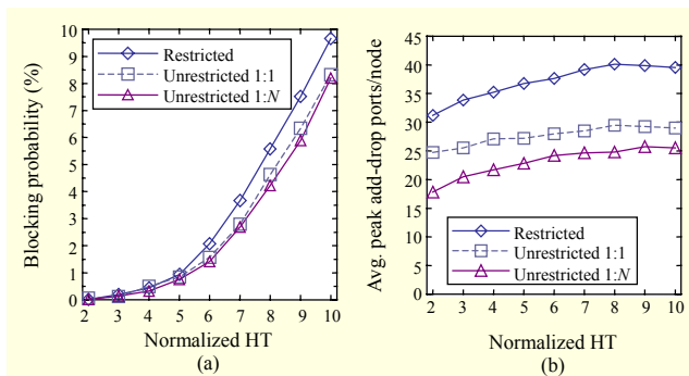
Fig. 3. (a) Average VON blocking probability and (b) peak add-drop port usage per node.
