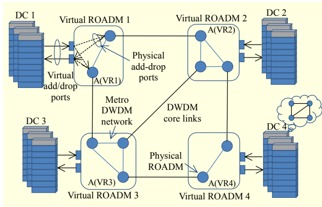
Fig. 1. VON for data center interconnection.
