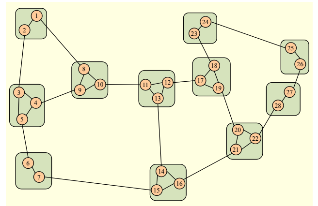
Fig. 2. Extended Abilene Internet2 network: 28 nodes, 37 bidirectional fiber links.
