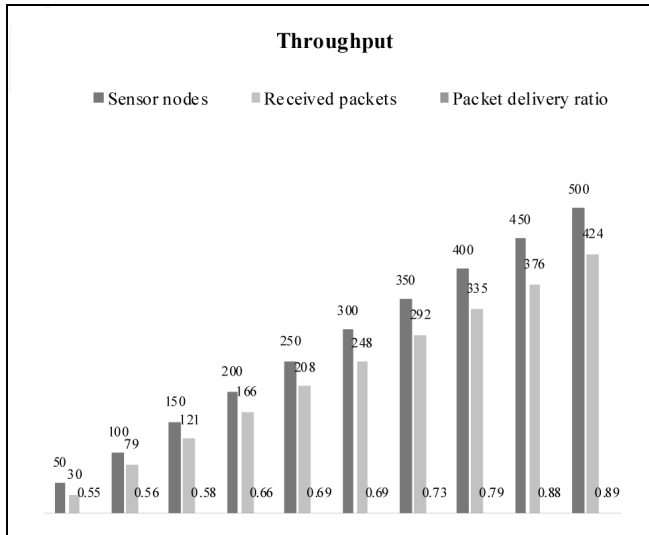
Fig.12. Throughput in terms of the packet delivery ratio
