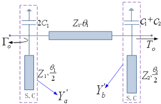
Figure6 Odd-mode excitation
