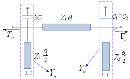
Figure 5: Even-mode excitation
