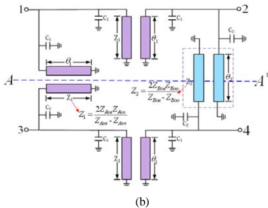
Figure 3: Reduced size ring hybrid circuit (a), equivalent circuit of ring hybrid with coupled line (b)
