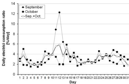
Figure 1: Average daily electric power consumption ratio of each month
