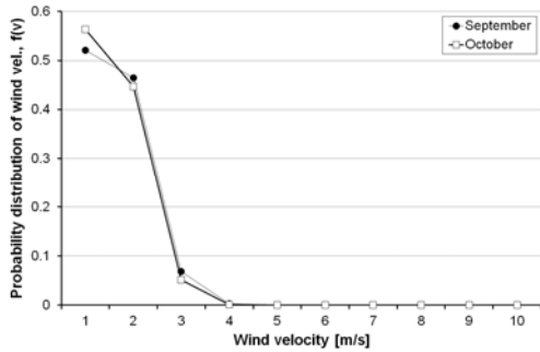
Figure 4: Weibull's probability distribution of wind velocity of each month
