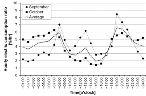
Figure 2: Average hourly electric power consumption ratio of each month
