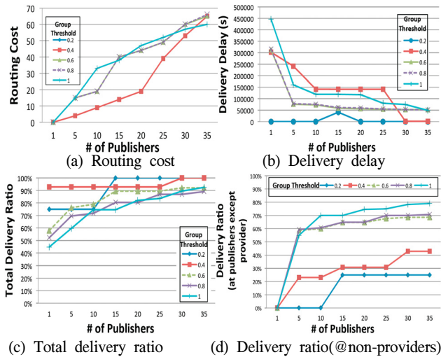
Fig. 2. Performance w.r.t group threshold and # of publishers.
