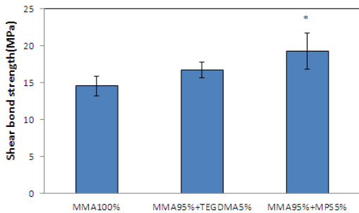
[Fig. 5] Shear bond strength of Vertex self resin on the surface treatment of silane coupling
