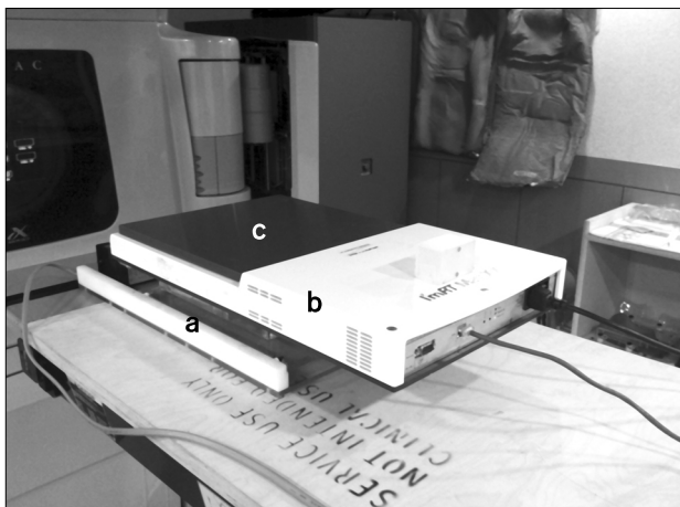
Fig. 1. Moving phantom consists of; (a) Moving platform, (b) I 1 m MatriXX, and (c) Solid water phantom. The platform moves by crank connected to the geared motor. This phantom designed to simulate respiratory-induced organ motion in craniocaudal direction.
