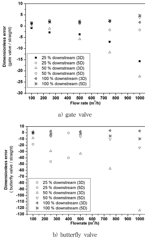
Fig. 8 Dimensionless error for various flow rate at the downstream (3D, 5D) of the gate valve and the butterfly valve
