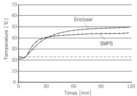
Fig. 7. Thermal test results.
