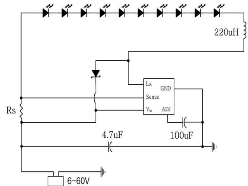
Fig. 3. Schematic diagram of LED driving circuit.
