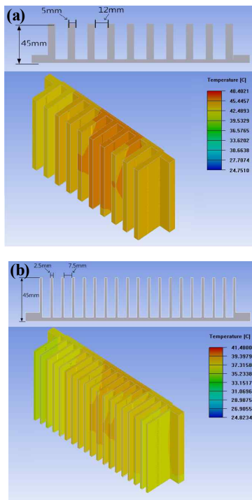
Fig. 4. Simulation results. (a) model 1, (b) model 2.
