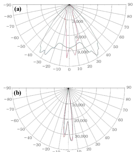
Fig. 10. Luminous distribution. (a) conventional, (b) LED.
