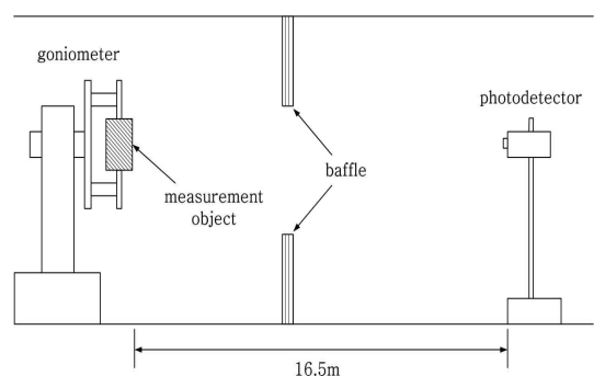
Fig. 9. Lay-out of a goniophotometer system.
