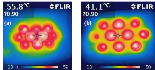
Fig. 5. Thermal distribution of LED package depending on array. (a) centralized type, (b) dispersal type.
