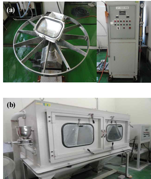
Fig. 11. Photograph of IP test equipment. (a) watering, (b) dusting.
