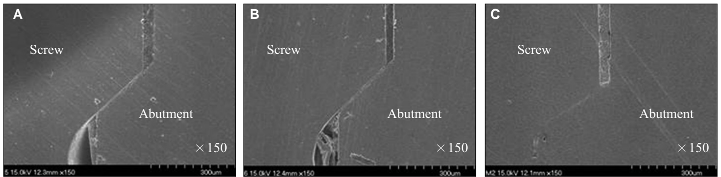
Fig. 7. FE-SEM ( \times 150 ) images of abutment-screw interface in each group. A: Ready-made abutment (Transfer abutment), B: CAD-CAM custom-made abutment (CustomFit abutment), C: CAD-CAM custom-made abutment (Myplant abutment).
