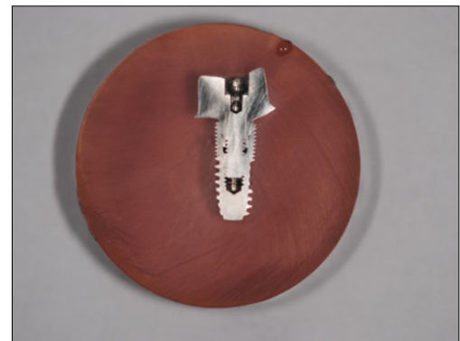
Fig. 5. Ground and polished specimen.
