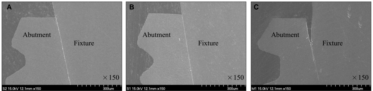
Fig. 6. FE-SEM ( \times 150 ) images of fixture-abutment interface in each group. A: Ready-made abutment (Transfer abutment), B: CAD-CAM custom-made abutment (CustomFit abutment), C: CAD-CAM custom-made abutment (Myplant abutment).
