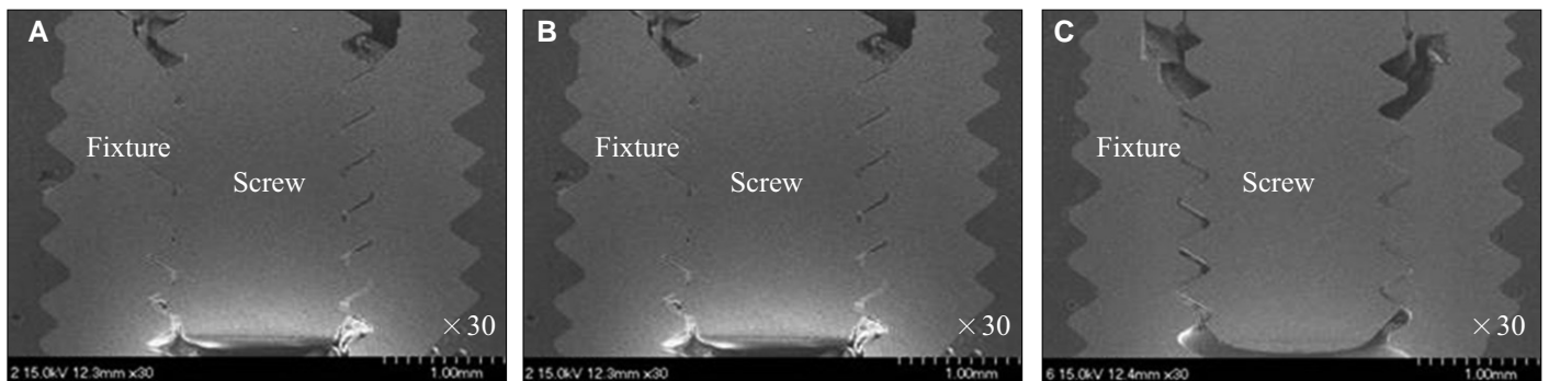
Fig. 8. FE-SEM ( \times 30 ) images of fixture-screw interface in each group. A: Ready-made abutment (Transfer abutment), B: CAD-CAM custom-made abutment (CustomFit abutment), C: CAD-CAM custom-made abutment (Myplant abutment).
