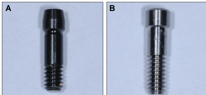
Fig. 3. Screws used in this study. A: Ready-made screw (Ebony gold, Osstem Implant Co. Ltd, Busan, Korea), B: CAD-CAM custom-made screw (Titanium, Raphabio Co., Seoul, Korea).
