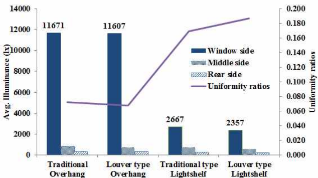
Fig. 6. Average illuminance and Uniformity ratios (Vernal equinox)
