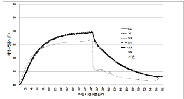
(a) 황토바닥재
