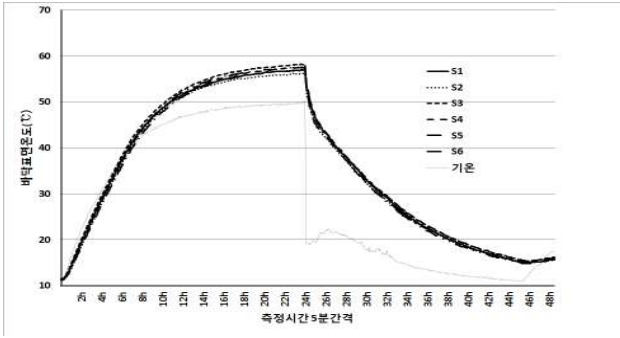
(a) 황토바닥재
