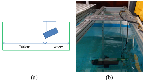
[Fig. 5] Installation of Sonar (a) Location of Sonar (b) Layout of Sonar & jig
