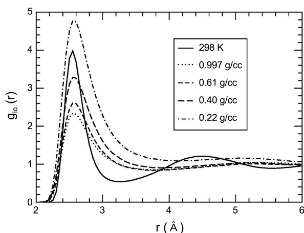
Figure 3. Radial distribution functions g_{io}(r) of SPC/E water molecules as a function of the distance r(\text{Å}) between OH - ( i ) and oxygen atom( o ) of a water molecule using q_O = -0.8476 e and q_H = +0.4238 e for OH - ion at 298 K (0.997 g/cc) and 673 K (0.997, 0.61, 0.40, and 0.22 g/cc).
