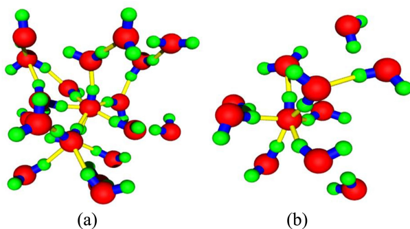
Figure 6. Snapshots of equilibrium configurations of SPC/E water molecules around \text{OH}^- ion within 5 Å using q_{\text{O}} = -2 e and q_{\text{H}} = +1 e for \text{OH}^- ion (Sim.2) at (a) T = 298 \text{ K} and (b) at T = 673 \text{ K} and \rho = 0.48 \text{ g/cc} .
