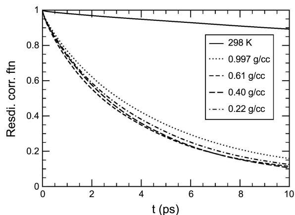
Figure 9. Residence time correlation function for the hydrated SPC/E water molecules in the first hydration shell of OH - ion using q_O = -2 e and q_H = +1 e for OH - ion (Sim.2) at 298 K (0.997 g/cc) and 673 K (0.997, 0.61, 0.40, and 0.22 g/cc).
