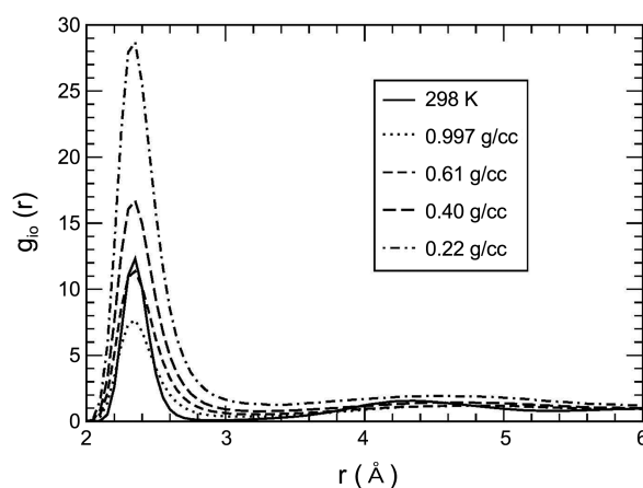
Figure 4. Radial distribution functions g_{io}(r) of SPC/E water molecules as a function of the distance r(\text{Å}) between OH - ( i ) and oxygen atom( o ) of a water molecule using q_O = -2 e and q_H = +1 e for OH - ion at 298 K (0.997 g/cc) and 673 K (0.997, 0.61, 0.40, and 0.22 g/cc).
