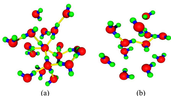
Figure 5. Snapshots of equilibrium configurations of SPC/E water molecules around \text{OH}^- ion within 5 Å using q_{\text{O}} = -0.8476 e and q_{\text{H}} = +0.4238 e for \text{OH}^- ion (Sim.1) at (a) T = 298 \text{ K} and (b) at T = 673 \text{ K} and \rho = 0.48 \text{ g/cc} .
