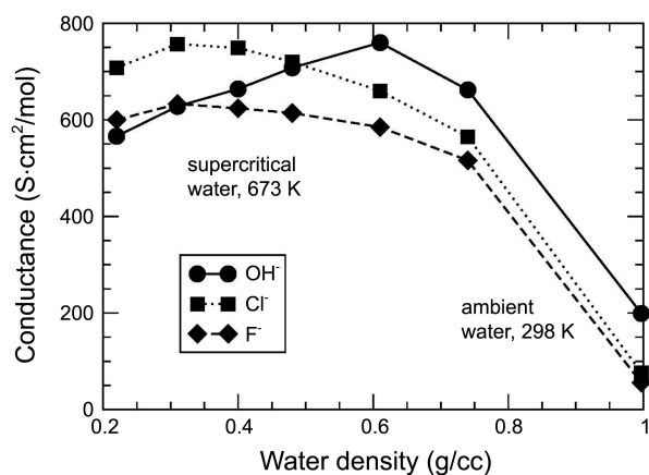
Figure 1. Limiting molar conductances of OH - , Cl - , and F - (assumed) ions as a function of water density in supercritical water and ambient water.
