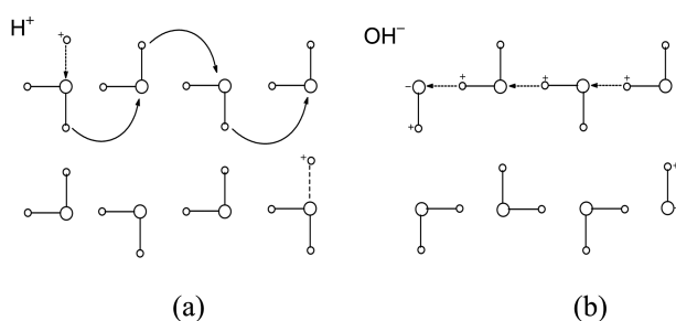
Figure 2. Grotthuss chain mechanisms.
