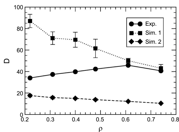
Figure 7. Comparison of diffusion coefficients D ( 10^{-5} \text{ cm}^2/\text{s} ) of \text{OH}^- ion as a function of water density (g/cc) calculated from the mean square displacement from MD simulations (Sim.1 ■: using q_{\text{O}} = -0.8476 e and q_{\text{H}} = +0.4238 e for \text{OH}^- ion, and Sim.2 ◆: using q_{\text{O}} = -2 e and q_{\text{H}} = +1 e for \text{OH}^- ion) with the experimental values (●). The error bars indicate the standard deviation.
