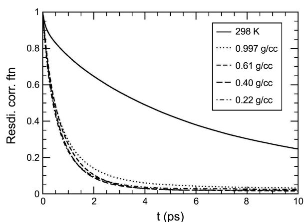
Figure 8. Residence time correlation function for the hydrated SPC/E water molecules in the first hydration shell of OH - ion using q_O = -0.8476 e and q_H = +0.4238 e for OH - ion (Sim.1) at 298 K (0.997 g/cc) and 673 K (0.997, 0.61, 0.40, and 0.22 g/cc) at 298 K (0.997 g/cc) and 673 K (0.997, 0.61, 0.40, and 0.22 g/cc).
