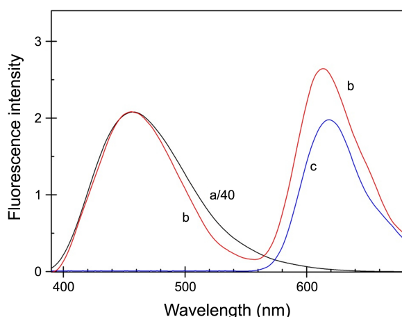
Figure 5. Emission spectrum of the DNA-DAPI adduct (curve a), DNA-DAPI- bis -Ru-bpp complex (curve b) and DNA- bis -Ru-bpp complex adduct (curve c). The samples were excited at 360 nm. Slit widths were 5 nm for both excitation and emission. [ Bis -Ru-bpp] = 1.2 \mu M, [DAPI] = 1 \mu M, [DNA] = 10 \mu M in nucleobase.
