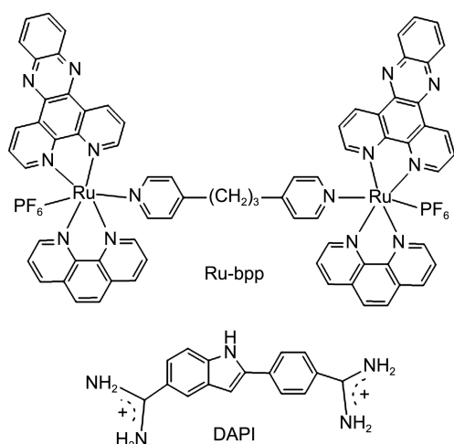
Figure 1. Chemical structure of the [\mu\text{-}(\text{linker})(\text{PF}_6)_2(\text{dipyrido}[3,2\text{-}a:2',3'\text{-}c]\text{phenazine})_2(\text{phenanthroline})_2\text{Ru(II)}_2]^{2+} with linkers: 1,3-bis-(4-pyridyl)-propane, abbreviated as bis -Ru-bpp and 4',6'-diamidino-2-phenylindole (DAPI).
