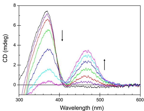
Figure 3. CD spectra of the DNA-DAPI-Ru-bpp complex adduct. [DAPI] = 10 \mu M, [DNA] = 100 \mu M in nucleobase. The concentrations of the bis -Ru-bpp complex increased to the arrow direction from 0 to 18 \mu M with an increment of 3 \mu M.
