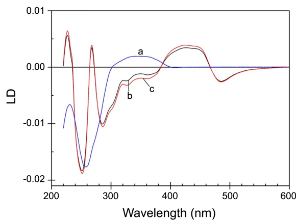
Figure 4. LD spectra of 18 \mu M concentration of the DNA-DAPI (curve a), the DNA- bis -Ru-bpp complex (curve b) and the DAPI- bis -Ru-bpp-DNA complex (curve c) adducts. [DAPI] = 10 \mu M, [DNA] = 100 \mu M in nucleobase. [ bis -Ru-bpp complex] = 18 \mu M.
