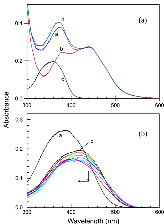
Figure 2. (a) Absorption spectra of bis -Ru-bpp and DAPI bound to DNA (curve b and curve c, respectively) and the DNA-DAPI- bis -Ru-bpp complex (curve a). Sum of curves b and c is denoted by curve d. [DNA] = 100 \mu\text{M} , [DAPI] = 6 \mu\text{M} and [ bis -Ru-bpp] = 18 \mu\text{M} . (b) Absorption spectrum of DAPI in the absence and presence of DNA (curve a and b, respectively), and the change in absorption spectrum of DNA-bound DAPI with increasing bis -Ru-bpp complex concentration (to arrow direction), which were constructed by subtraction of the absorption spectra the DNA- bis -Ru-bpp complex from that of the DNA-DAPI- bis -Ru-bpp complex. [DNA] = 100 \mu\text{M} , [DAPI] = 10 \mu\text{M} , [ bis -Ru-bpp] = 0-18 \mu\text{M} . The bis -Ru-bpp complex increased with an increment of 3 \mu\text{M} .
