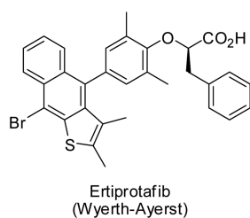
Figure 1. The structure of Ertiprotafib.
