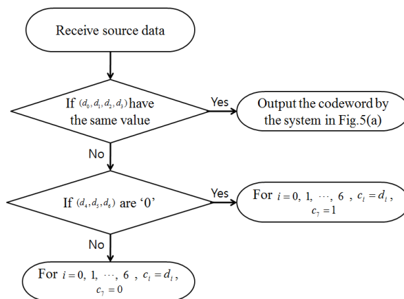
Fig. 4. Encoding procedure.
