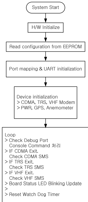
Figure 8 : Initializing Processor
