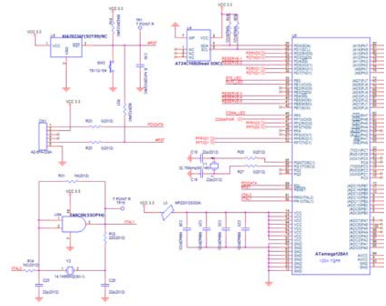
Figure 4 : The design circuits using ATxmega128A1
