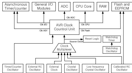
Figure 3 : The diagram of a clock and distribution in ATxmega128A1
