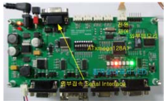
Figure 2 : The photograph of the fabricated signal processing board for hybrid communication
