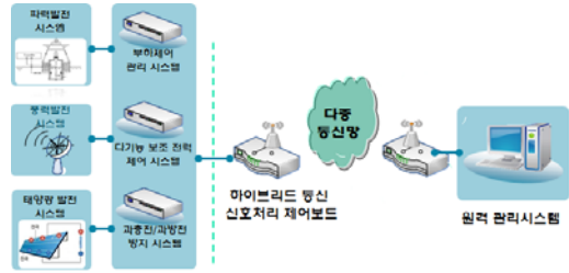
Figure 1 : The blockdiagram of the Tele-controller system of navigational aids using hybrid communication
