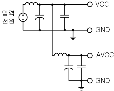
Figure 5 : Decoupling Circuits
