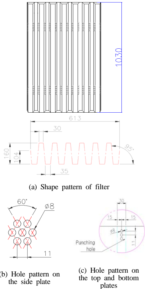
Figure 3: Shape details of the filter (perforated plate) installed in the strainer
