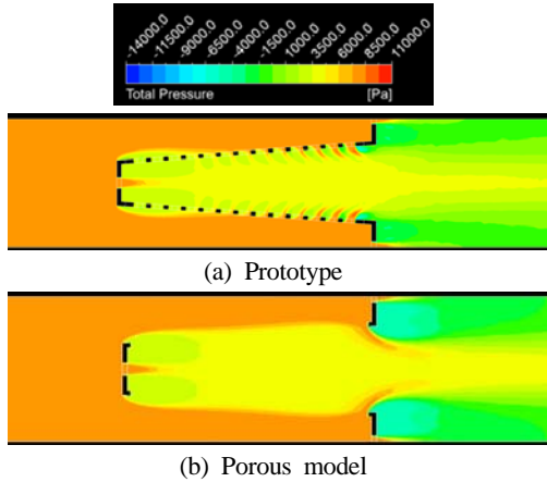
Figure 8: Distributions of total pressure on a horizontal cross section obtained from the numerical simulations on the unit shape pattern of the strainer
