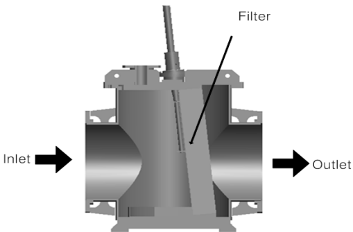
Figure 2: View on a certain vertical cross section of the strainer
