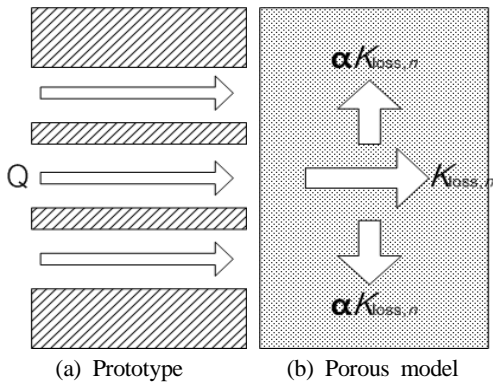
Figure 1: Schematic illustrating the prototype and porous model for the numerical simulation on a strainer
