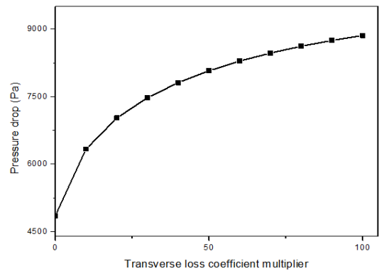
Figure 5: Variation of the pressure drop with the transverse loss coefficient multiplier for the unit shape pattern of the strainer
