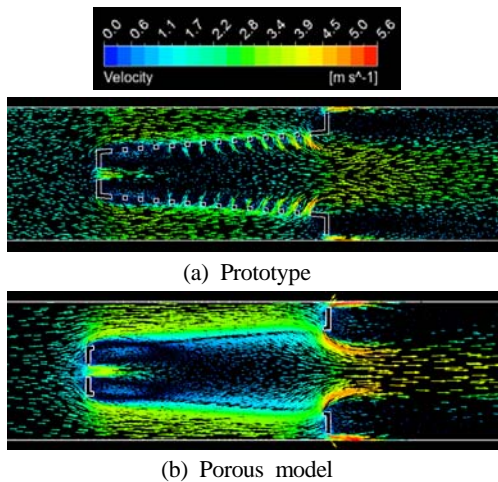
Figure 9: Distributions of flow velocity on a horizontal cross section obtained from the numerical simulations on the unit shape pattern of the strainer
