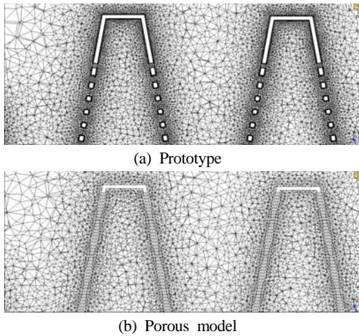
Figure 11: Meshes generated around the filter for the numerical simulations on the whole shape pattern of the strainer
