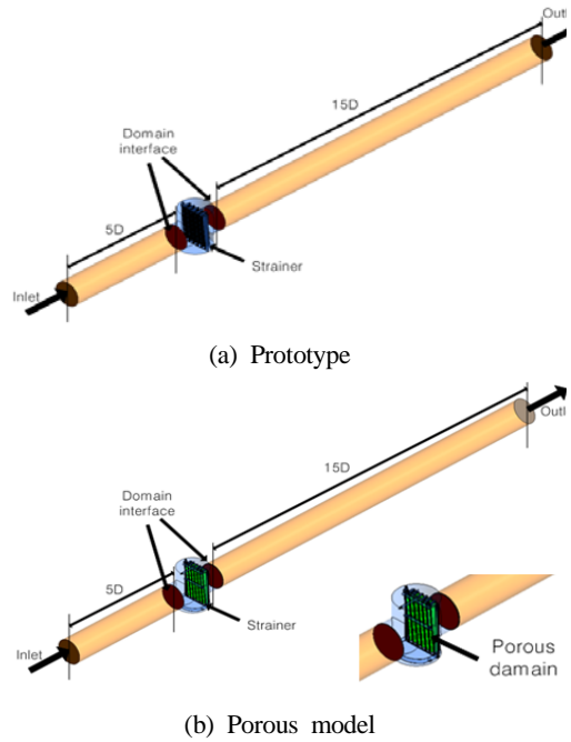
Figure 10: Schematics illustrating the computational domains for the numerical simulations on the whole shape pattern of the strainer
