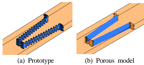
Figure 4: Unit shape pattern of filter simulated to obtain the transverse loss coefficient in the strainer
