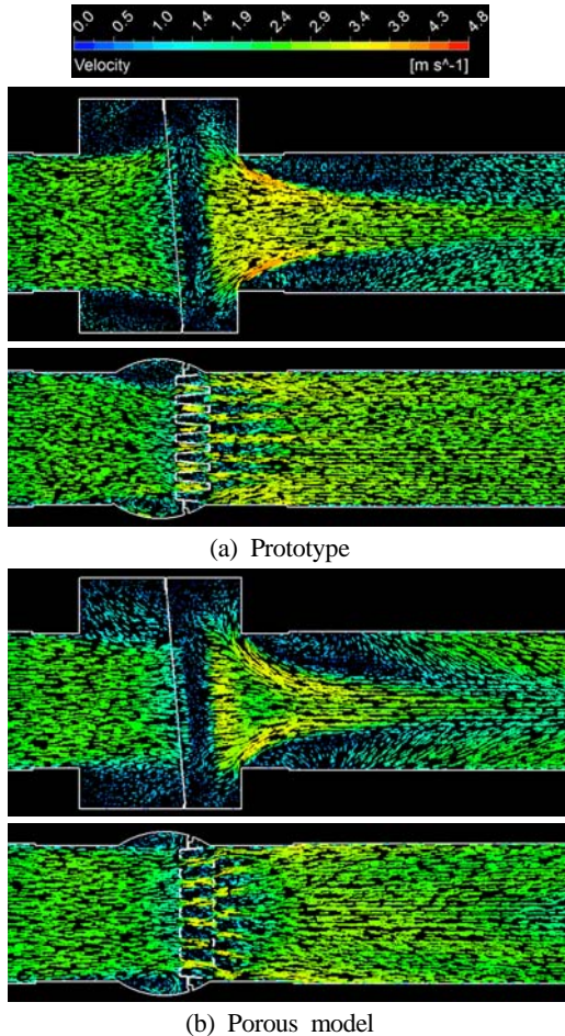
Figure 13: Distributions of flow velocity on certain vertical (upper) and horizontal (lower) cross sections obtained from the numerical simulations on the whole shape pattern of the strainer
