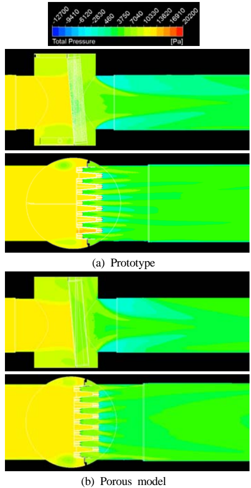
Figure 12: Distributions of total pressure on certain vertical (upper) and horizontal (lower) cross sections obtained from the numerical simulations on the whole shape pattern of the strainer
