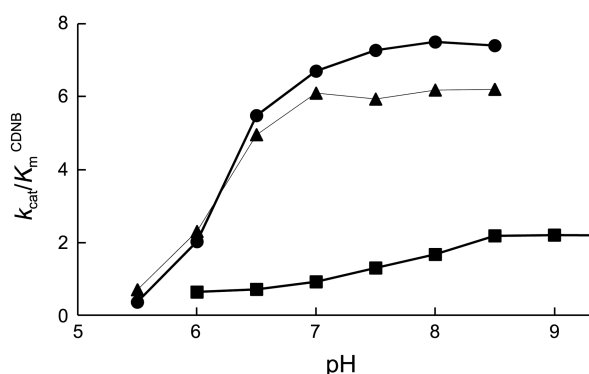
Figure 3. Dependence of k_{cat}/K_m^{CDNB} values on pH. The kinetic parameters of OsGSTF3 , Y8F and Y8A for the conjugation of GSH with CDNB were determined under the conditions of saturating GSH (2.5 mM) and variable concentrations of CDNB (0.1–1.0 mM). ●, OsGSTF3 ; ▲, Y8F; ■, Y8A.
