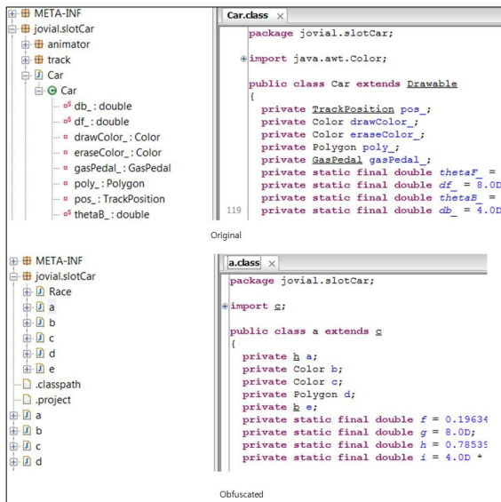
Fig. 11. Comparison before and after applying Proguard obfuscator
