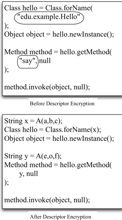
Fig. 13. Example of String Encryption and API Hiding
