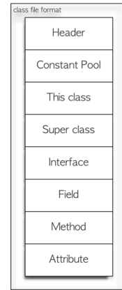
Fig. 1. Class file format
