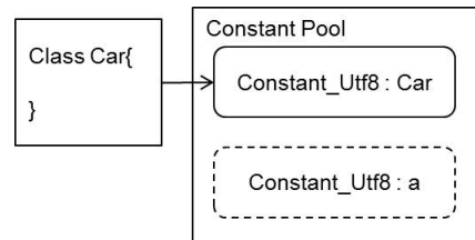
Fig. 8. Step 1: adding a renamed identifiers into constant pool
