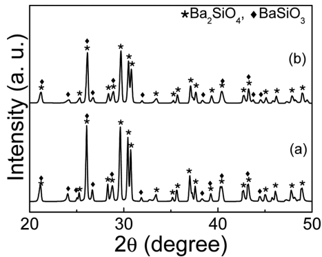
Fig. 3. XRD patterns of the samples prepared at 1300°C with prior calcination at 900°C. (a) sol-gel and (b) hybrid. (1.2 M TEOS).
