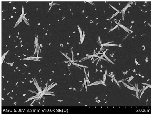
Fig. 7. SEM micrograph of B_2S:Eu^{2+} powders prepared by the hybrid process with prior calcination at 1000°C. (1.1 M TEOS).
