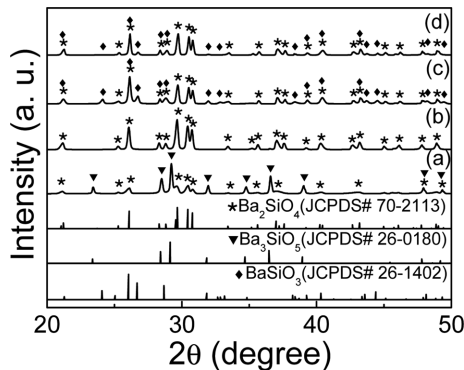
Fig. 1. XRD patterns of the samples prepared at 1300°C without calcination with different amounts of TEOS of (a) 1.0 M, (b) 1.2 M, (c) 1.4 M, and (d) 1.2 M. [(a) - (c): sol-gel; (d): hybrid].
